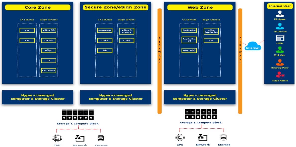
Logical Setup at DR- Jaipur
